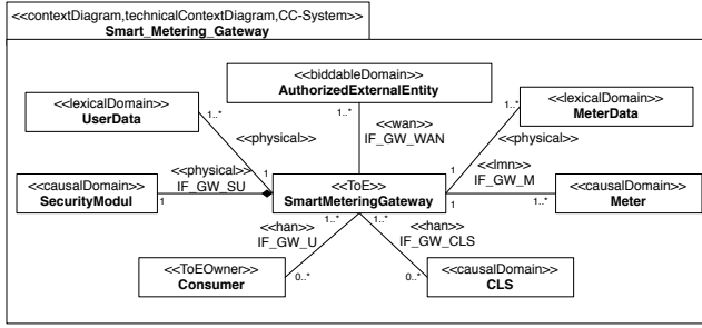
Figure 2: The Context Diagram of the Smart Metering Gateway
