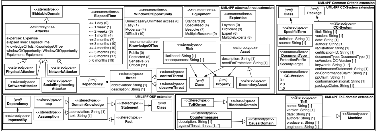
Figure 1: A Common Criteria extension of the UML4PF Profile
